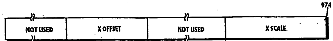
Fig. 35M VIDEO INTERFACE X SCALE REGISTER (R/W)
